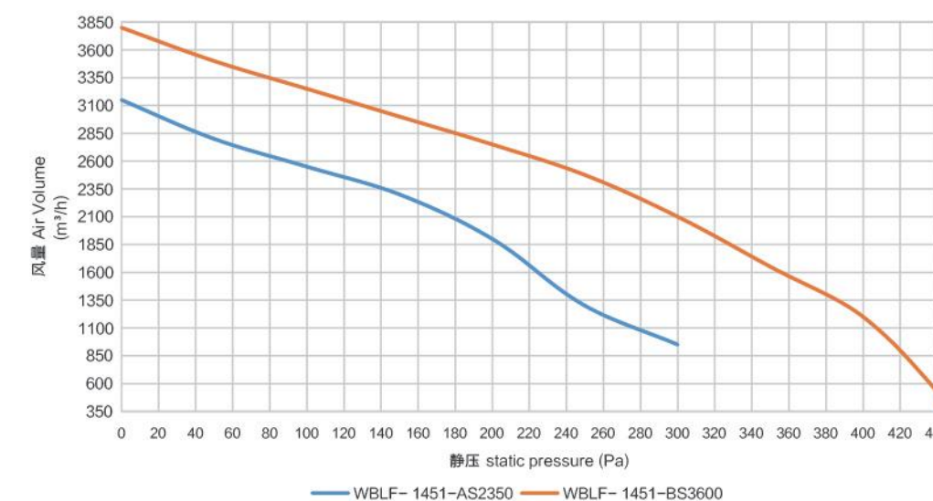
风量曲线图 Performance Curve
