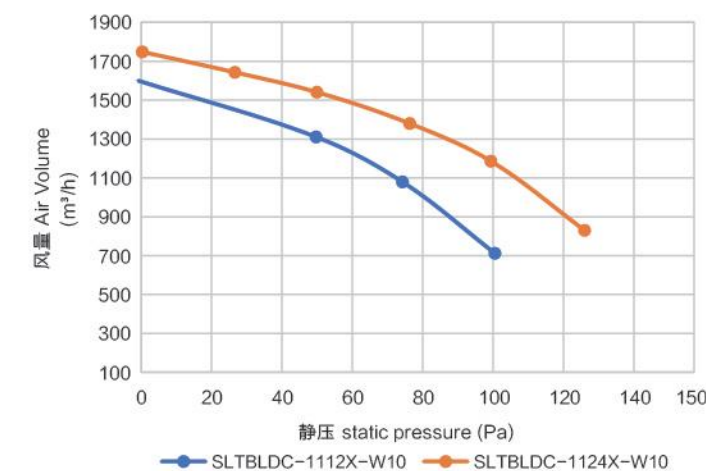
风量曲线图 Performance Curve
