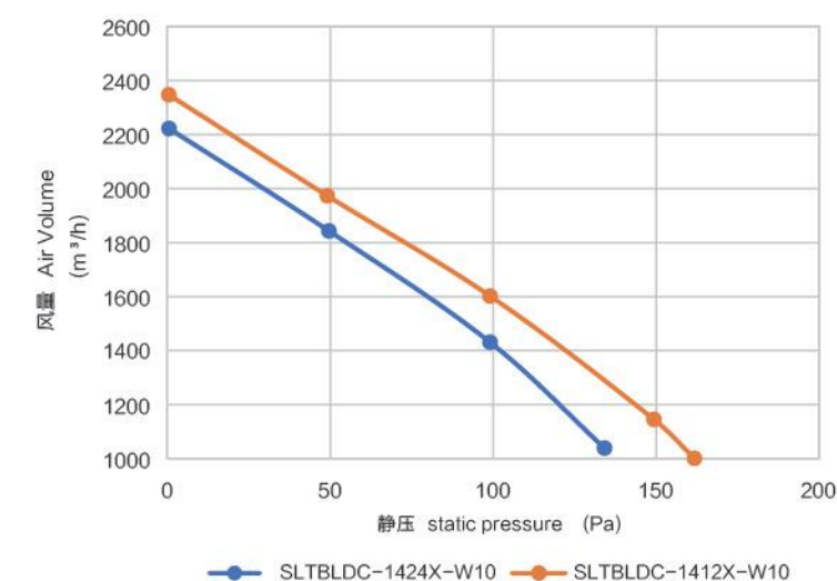
风量曲线图 Performance Curve
