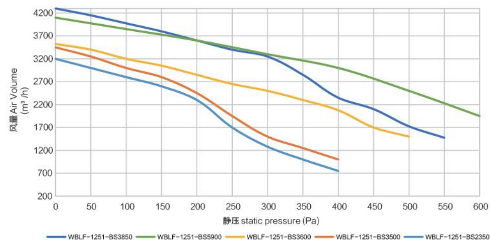
风量曲线图 Performance Curve
