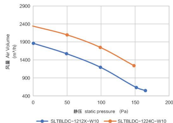
风量曲线图 Performance Curve
