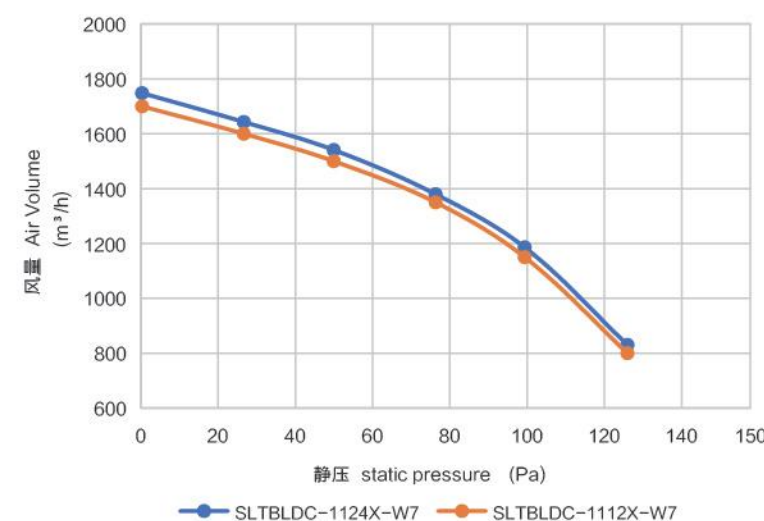
风量曲线图 Performance Curve
