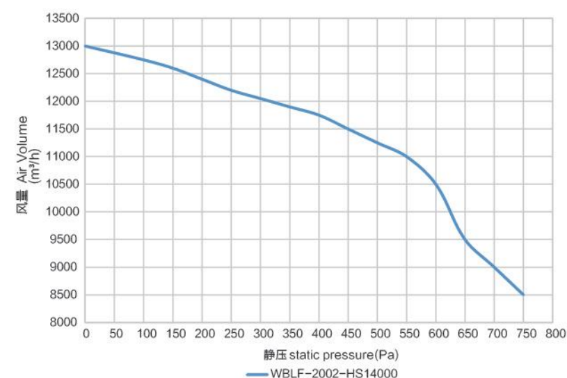
风量曲线图 Performance Curve
