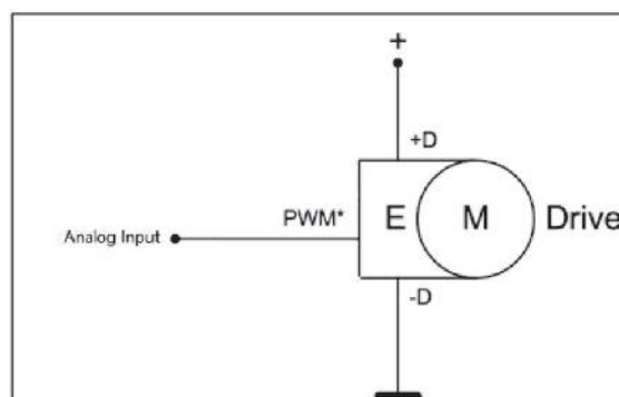
模拟电压调速 Analog control
